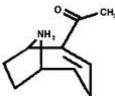
Figure 3. Structure of anatoxin-a
